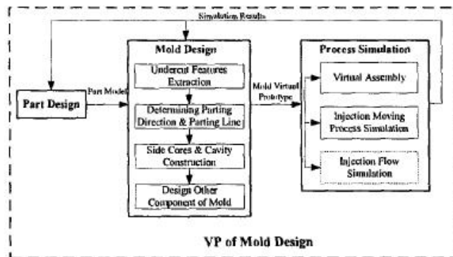
Fig. 1. Overall framework of VP for mold design
