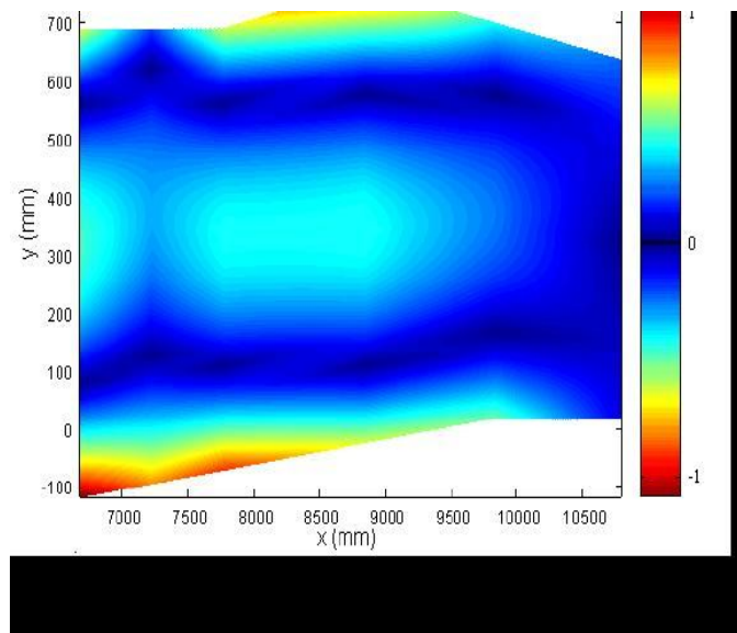
(b) Error distribution result after surface analysis
