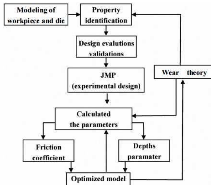
Figure 2. The process flow of die-related design
