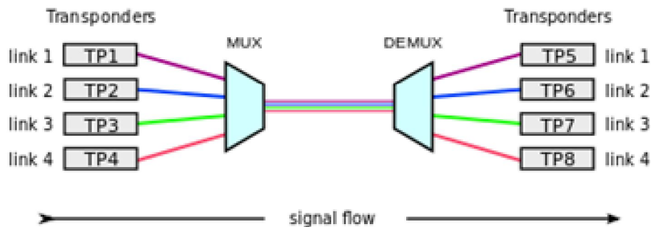
Fig1: A schematic diagram of WDM
