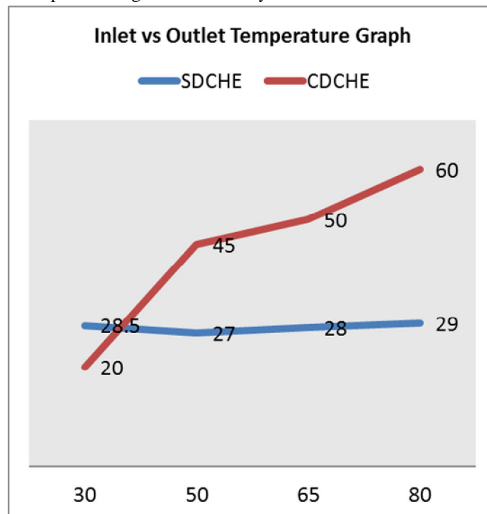
Fig. 3. Test run performance graph between common direct contact heat exchanger and specialized direct contact heat exchanger
