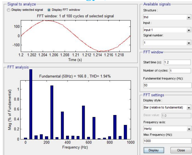
Fig.5THD
