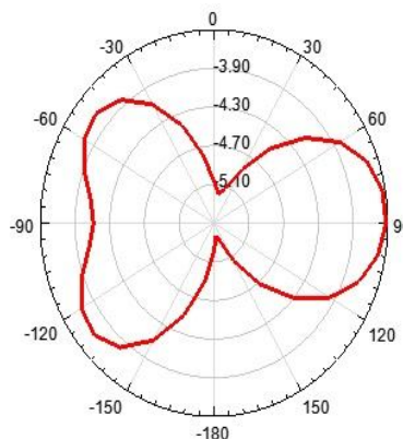
Figure 8 Azimuthal pattern (H-plane) gain display (for \phi = \text{all values} and \theta = 90 degree)
