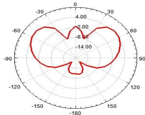
Figure 11 Elevation pattern (E-Plane) gain display (for \theta =all values and \phi = 0 degree)
