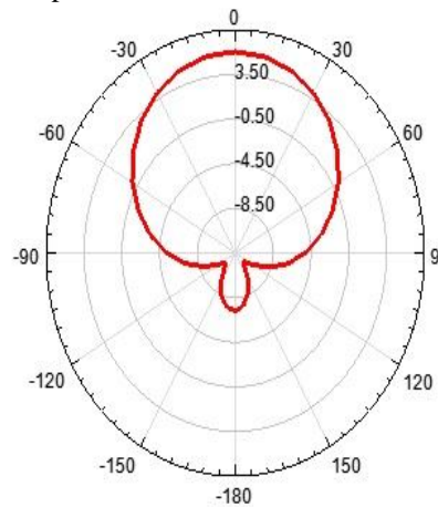
Figure 7 Elevation pattern (E-Plane) gain display (for \theta = \text{all values} and \phi = 0 degree)
