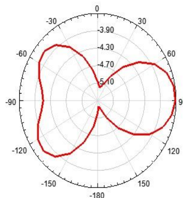
Figure 8 Azimuthal pattern (H-plane) gain display (for \phi = all values and \theta = 90 degree)
