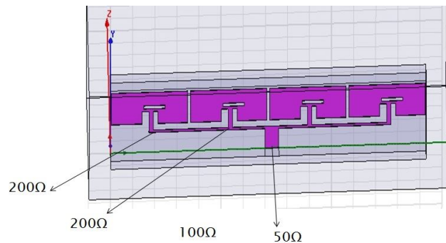
Figure 4 Simulated dual band array antenna design
