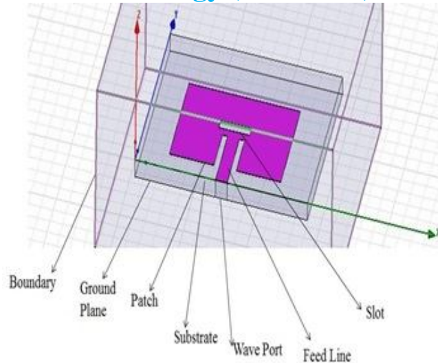
Figure 2 Simulated geometry of dual band antenna design
