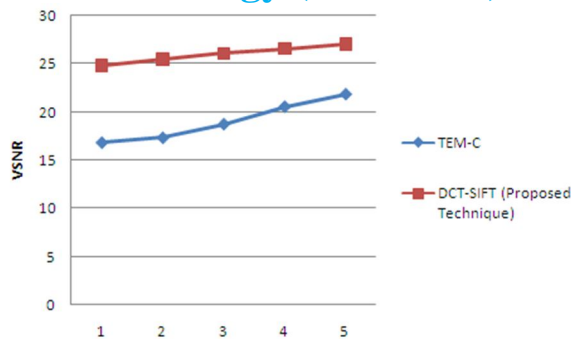
Fig 6: Comparison of VSNR for image size 256x384
