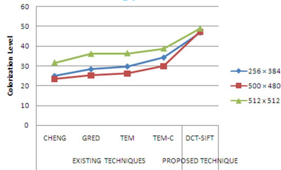
Fig 11: Comparison of Colorization Level for different image sizes
