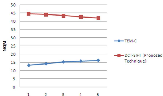
Fig 8: Comparison of NQM for image size 256x384
