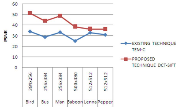
Fig 9: Comparison of PSNR for different image sizes
