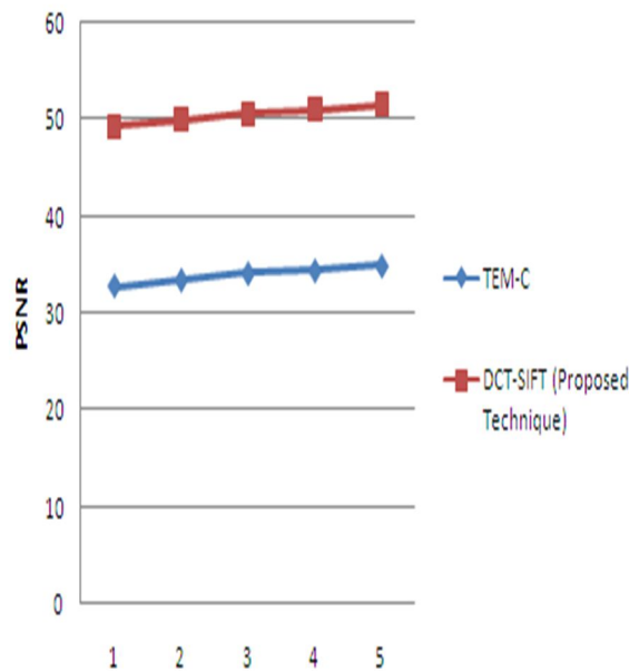
Fig 5: Comparison of PSNR for image size 256x384
