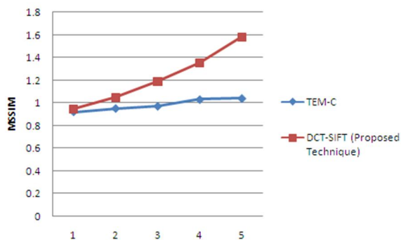
Fig 7: Comparison of MSSIM for image size 256x384
