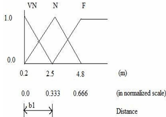
Figure. 2 Membership function of distance used in fuzzy approach
