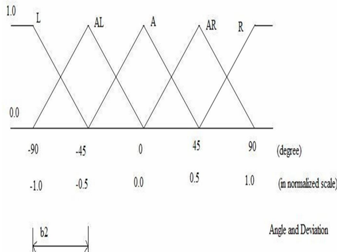
Figure. 3 Membership function of angle used in fuzzy approach
