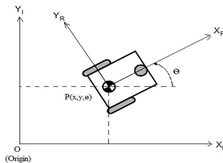
Figure. 1 The global reference frame and the mobile robot local reference frame.
