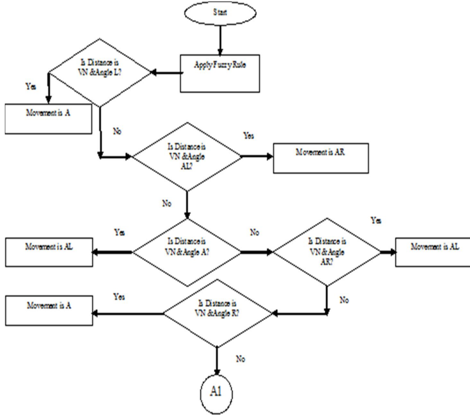
Flow chart of possible rules used in an algorithm
