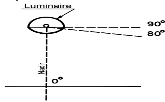
Fig 2 The candlepower of luminaires designated as full-cutoff, cutoff, and semi cutoff is limited at angles of 90 and 80 degrees from the nadir
