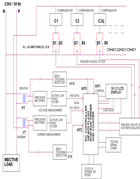
Fig.1 Block Diagram
