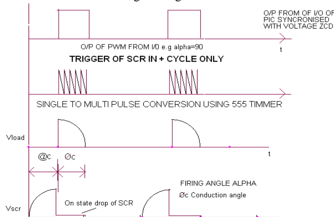
Fig7.Trigger for SCR
