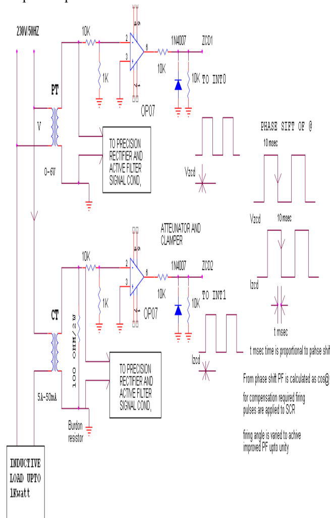
Fig 3.ZCD block for phase shift measurement
