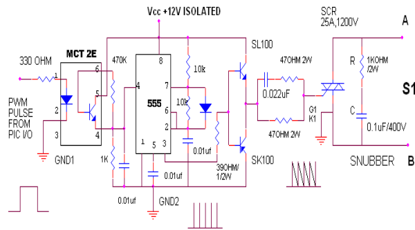
Fig6.Firing circuit
