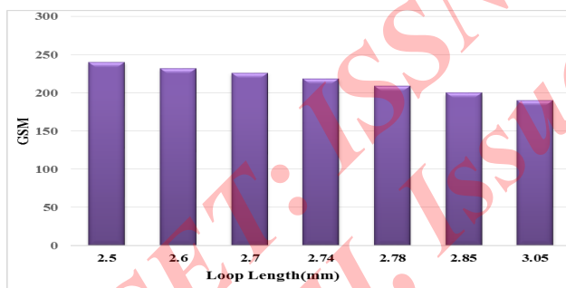
Fig. 1 Change of GSM of fabric with Loop length
